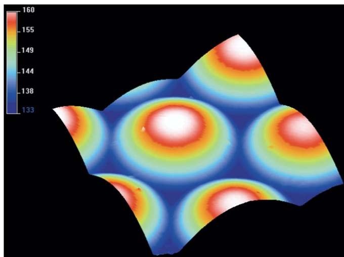
Fig. 6: Topography of a microlens array in a 1 \times 1 \text{ mm}^2 area. The scale shows the object height in \mu\text{m} .
